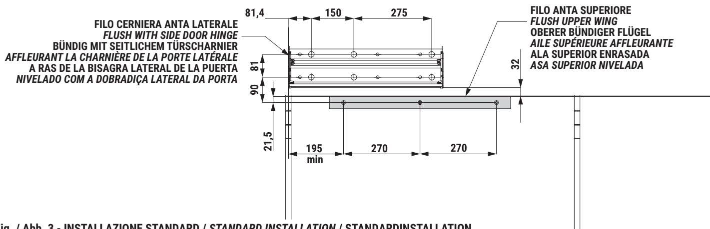
Fig. / Abb. 3 - INSTALLAZIONE STANDARD / STANDARD INSTALLATION / STANDARDINSTALLATION INSTALLATION STANDARD / INSTALACIÓN ESTÁNDAR / INSTALAÇÃO STANDARD
