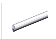
BA/90/2 White painted aluminum rod, 2 meters long, with LED cover profile and impact resisting rubber profile.
