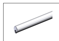
BA/90/6 White painted aluminum rod, 6 meters long, with LED cover profile and impact resisting rubber profile.
